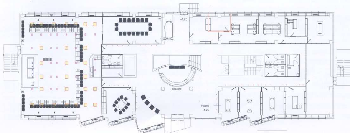
PIANO TERRA - IMAP
